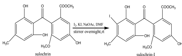
Fig. 1. Reaction of sulochrin-I.
