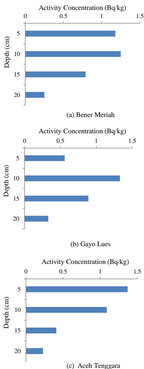
Fig. 3. Depth distribution of ^{137}\text{Cs} activity concentration in soils of areas unaffected by the tsunami (a) Bener Meriah, (b) Gayo Lues and (c) Aceh Tenggara.
