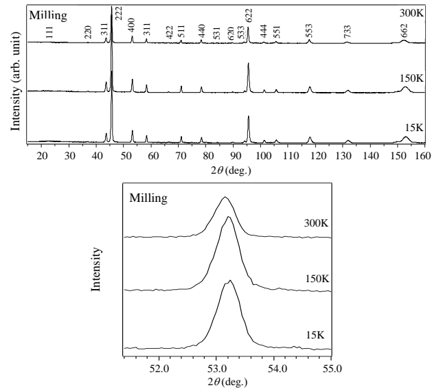
Fig. 6. Neutron diffraction patterns taken from HRPD-HANARO of the spinel-type \text{LiMn}_2\text{O}_4 synthesized with an initial molar ratio of \text{Li}/\text{Mn} = 0.50 by MA method and annealed at 800^\circ\text{C} for 4 hours in \text{O}_2 then cooled with cooling rate of 60^\circ\text{C}/\text{h} . (a) whole pattern and (b) (400) peaks.
