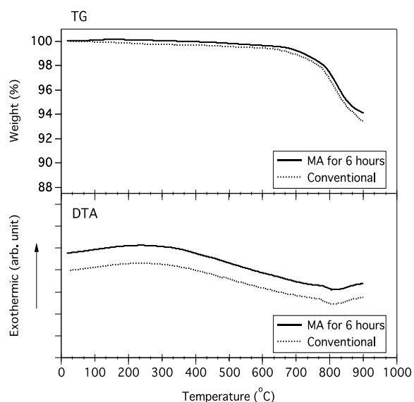
Fig. 2. TG-profiles and DTA-curves of the mixture of \text{LiOH}\cdot\text{H}_2\text{O} and \text{MnO}_x with an initial molar ratio of \text{Li}/\text{Mn} = 0.50 synthesized by MA for 6 hours and conventional method and subsequent annealing at 800 °C for 4 hours in \text{O}_2 with cooling rate of 60 °C/h.
