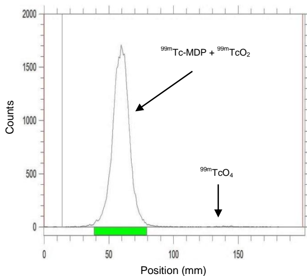
Fig. 1. Radiochromatogram of 99m Tc-MDP using acetone as mobile phase.
