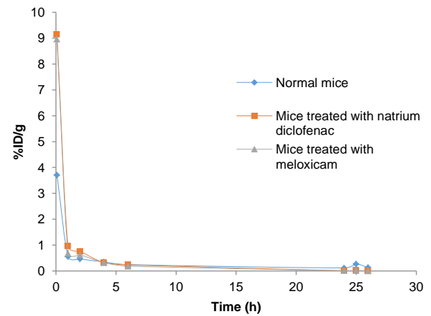
Fig. 3. Pharmacokinetic profile of 99m Tc-MDP in mice treated by sodium diclofenac and meloxicam.
