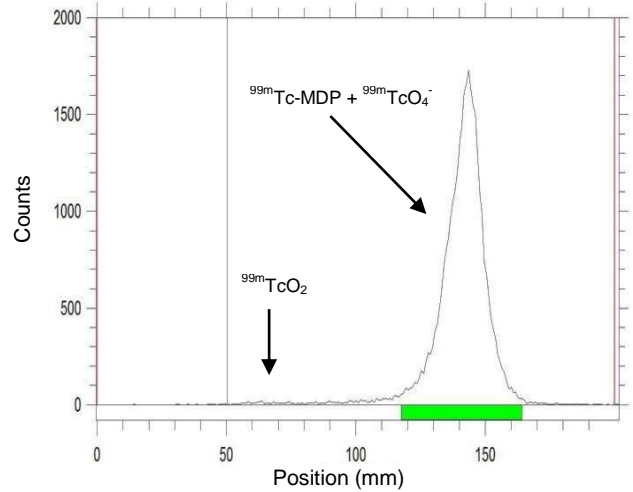
Fig. 2. Radiochromatogram of 99m Tc-MDP using saline solution as mobile phase.
