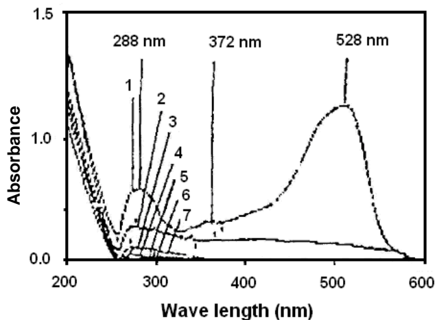
Figure 13. Absorption spectra of irradiated Direct Red in O 2 bubbling solutions ( 1= 0 kGy; 2= 0.5 kGy; 3= 1 kGy; 4=1.5 kGy; 5= 2 kGy; 6 = 3 kGy and 7= 4 kGy)
