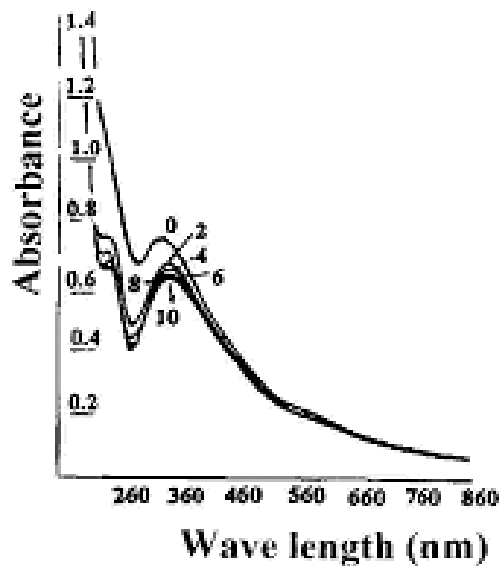
Figure 8. Absorption spectra of irradiated TB BGE in O 2 bubbling solutions (0,2,4,6,8, and 10 represent the dose in kGy).
