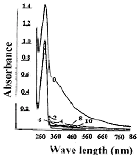
Figure 9. Absorption spectra of irradiated TB BGE in O 2 bubbling solutions + HNO 3 ( 0,2,4,6,8,10 and 12 represent the dose in kGy).
