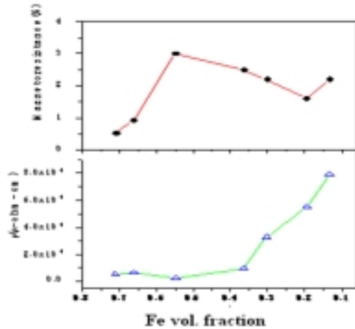
Figure 6. Resistivity and Magnetoresistance ratio of Fe-Al 2 O 3 granular film as a function of Fe volume fraction.
