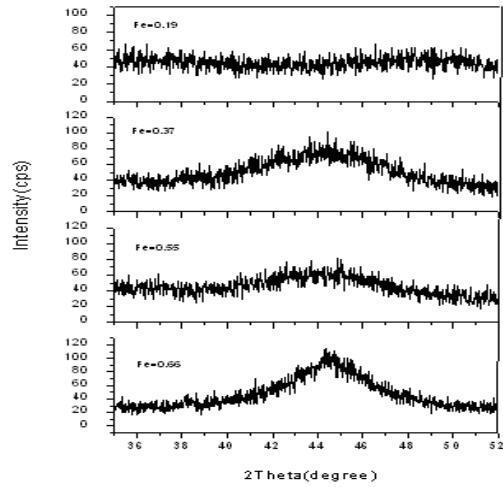
Figure 1. The peaks correspond to the Fe[110] as a function of Fe volume fraction in Fe-Al 2 O 3 granular film and its crystallite size d.
